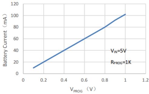
Battery Current vs. V_{PROG}
