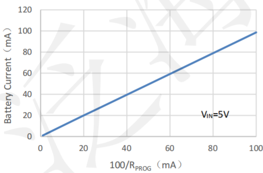
Battery Current vs. R_{PROG}
