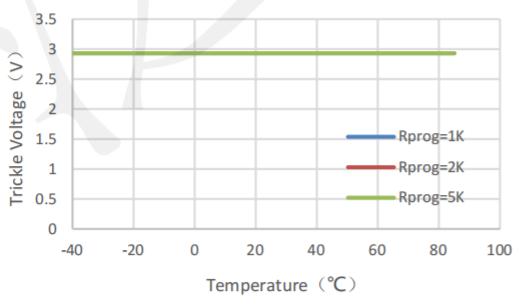
Trickle Voltage vs. Temperature
