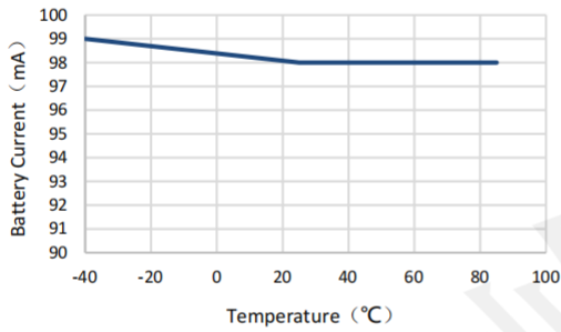
Battery Current vs. Temperature
