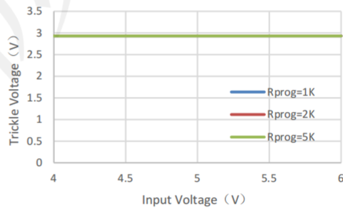
Trickle Voltage vs. Input Voltage
