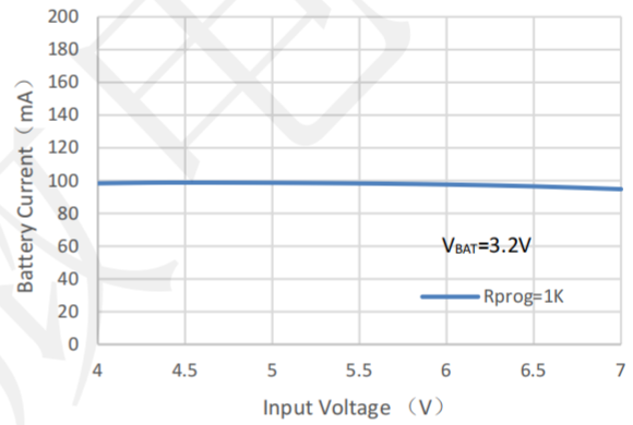
Battery Current vs. Input Voltage
