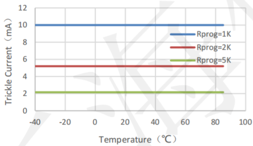
Trickle Current vs. Temperature
