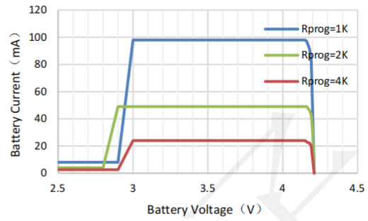
Battery Current vs. Battery Voltage
