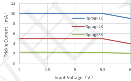
Trickle Current vs. Input Voltage
