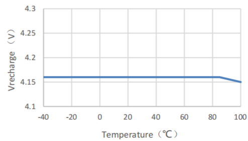
Vrecharge vs. Temperature (4.35V)
